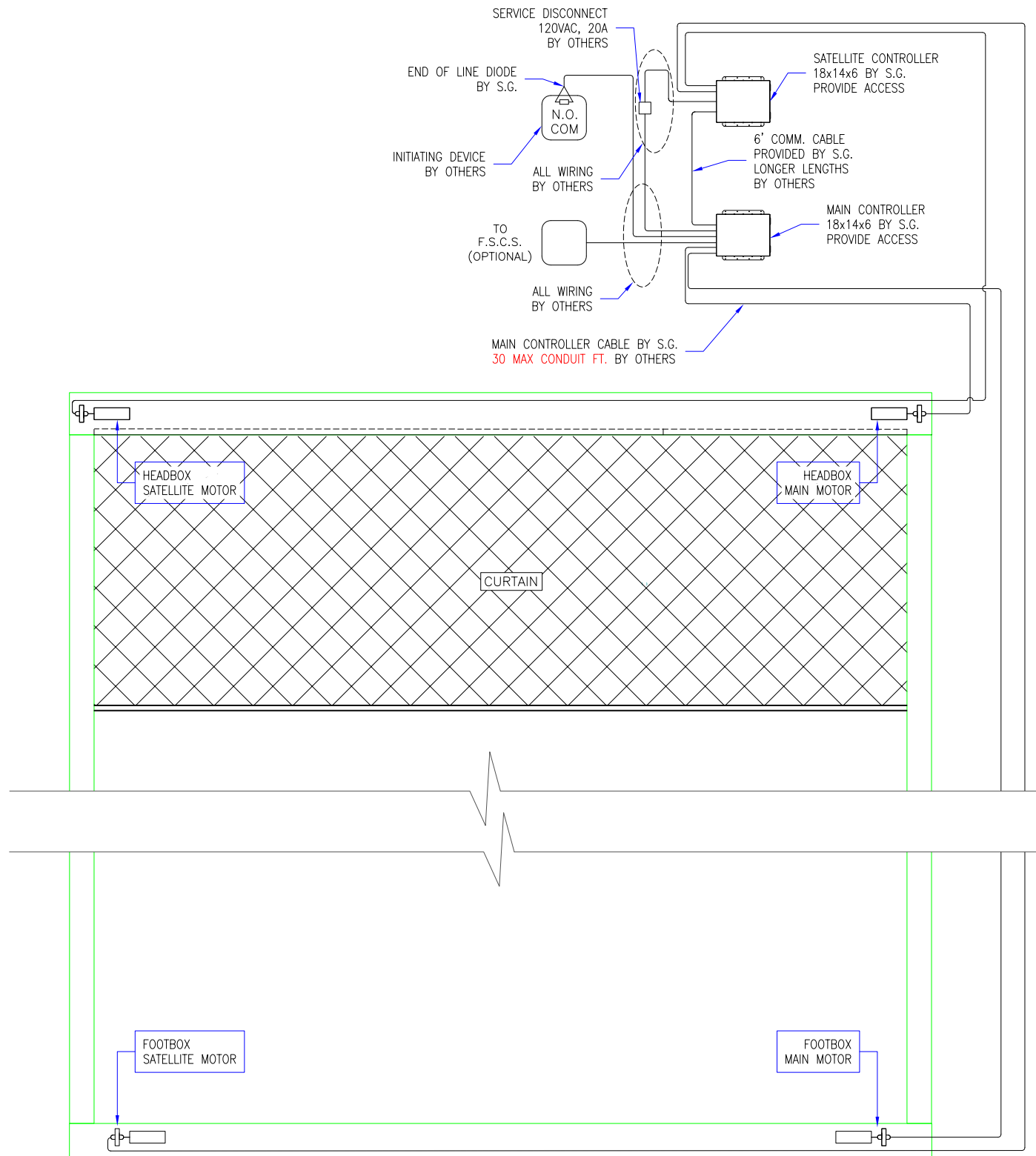
1 M3000 ELECTRICAL DETAILS SCALE: 1/4" = 1'-0"
